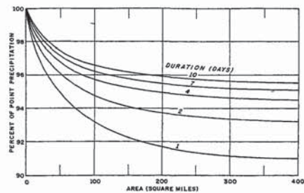
FIGURE 10.—Depth-area curves.
