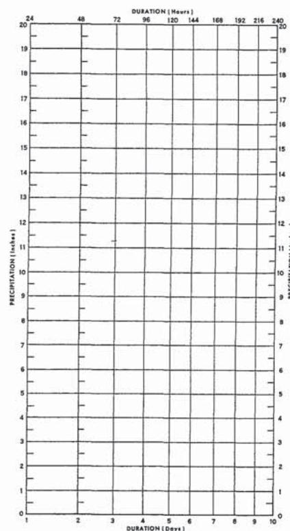
FIGURE 3.—Duration-interpolation diagram.
