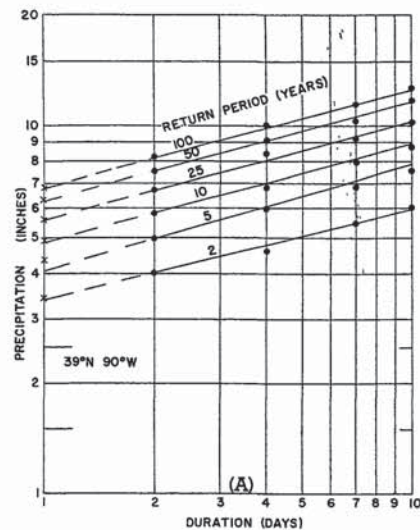
FIGURE 9.—Smoothing values read from isopluvial maps. Points are values read from maps of figures 12 to 35 for (A) 39°00' N., 90°00' W., and (B) 40°30' N., 111°15' W. The x's are values obtained from the maps of [1].
