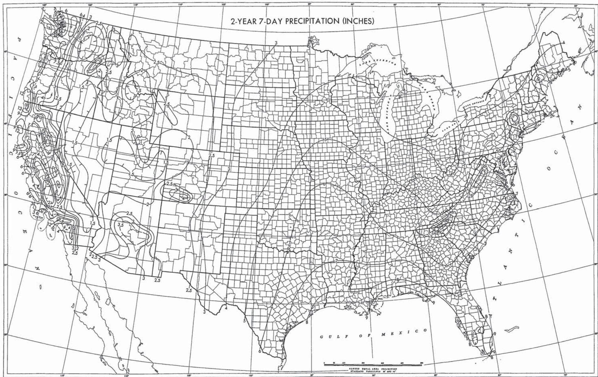
FIGURE 24.—2-year 7-day precipitation (in.).
