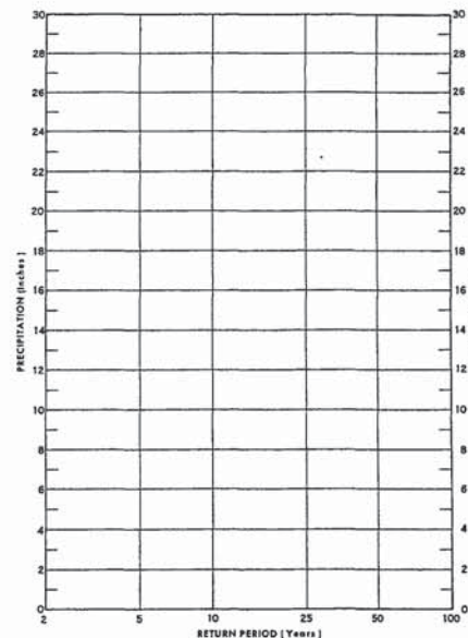
FIGURE 5.—Return-period-interpolation diagram.
